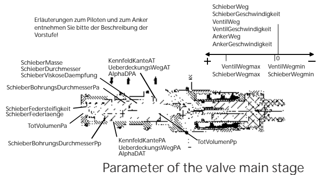
Cross Section view of the valve
